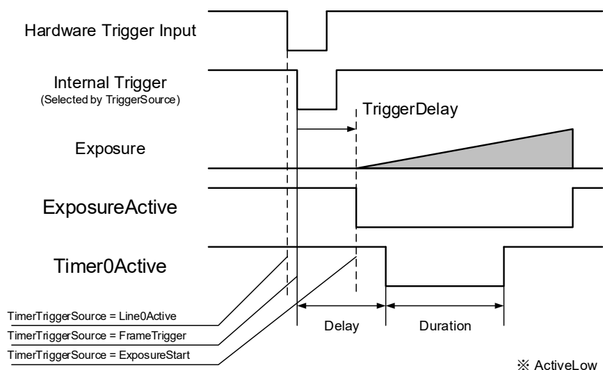
Fig. Timer0Active
