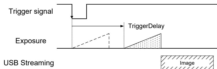
Fig. Trigger Delay
