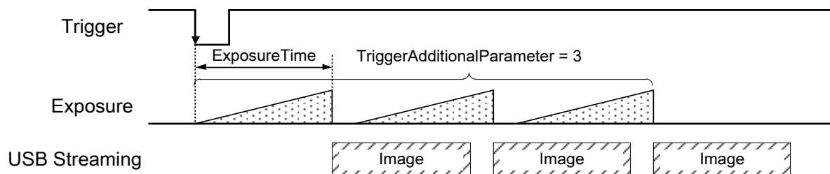
Fig. Trigger sequence
