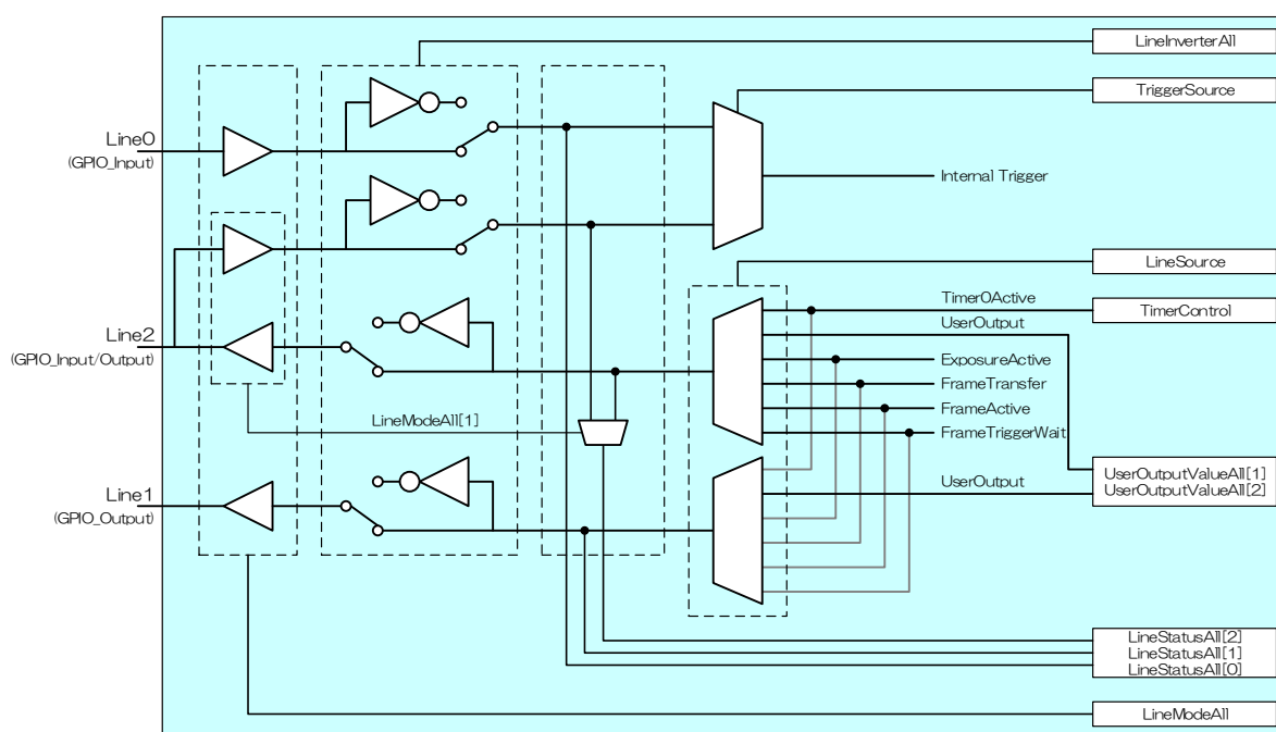
Fig. GPIO internal circuit diagram
