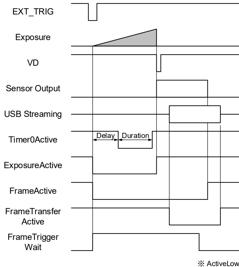
Fig. Selectable signals
